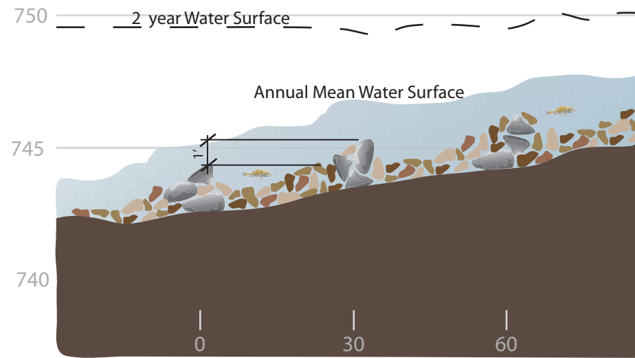
Bypass Profile through center of channel Scale: 1 in Horizontal = 25 ft 1 in Vertical = 5 ft
