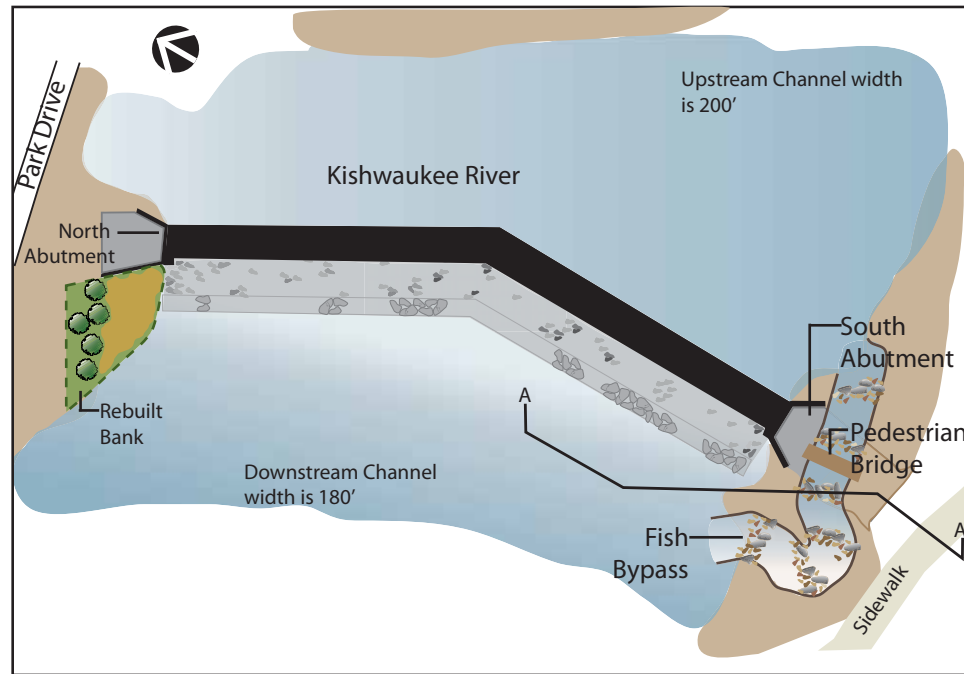
Plan View of Bypass Not to Scale
